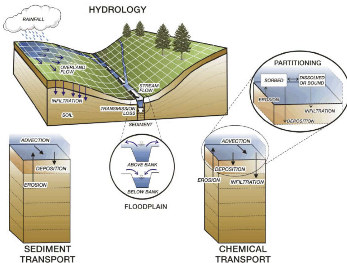
Figure 3. TReX model overview for hydrologic, sediment transport and chemical transport processes
